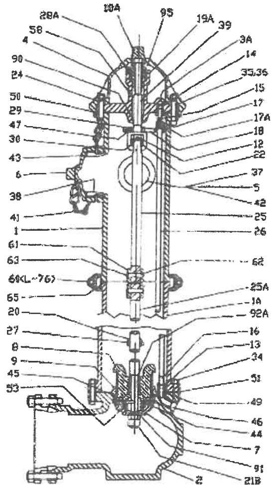
STANDARD HYDRANT AP SMITH #L-76
