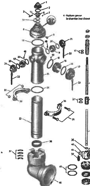
Safety Flange Repair Kit
